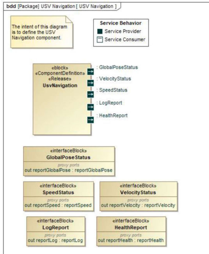
Figure 5. UAA SDK USV Navigation
