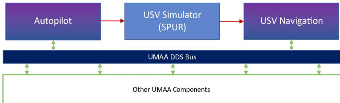
Figure 4. UMAA SDK Autopilot and USV Navigation Components with SPUR
